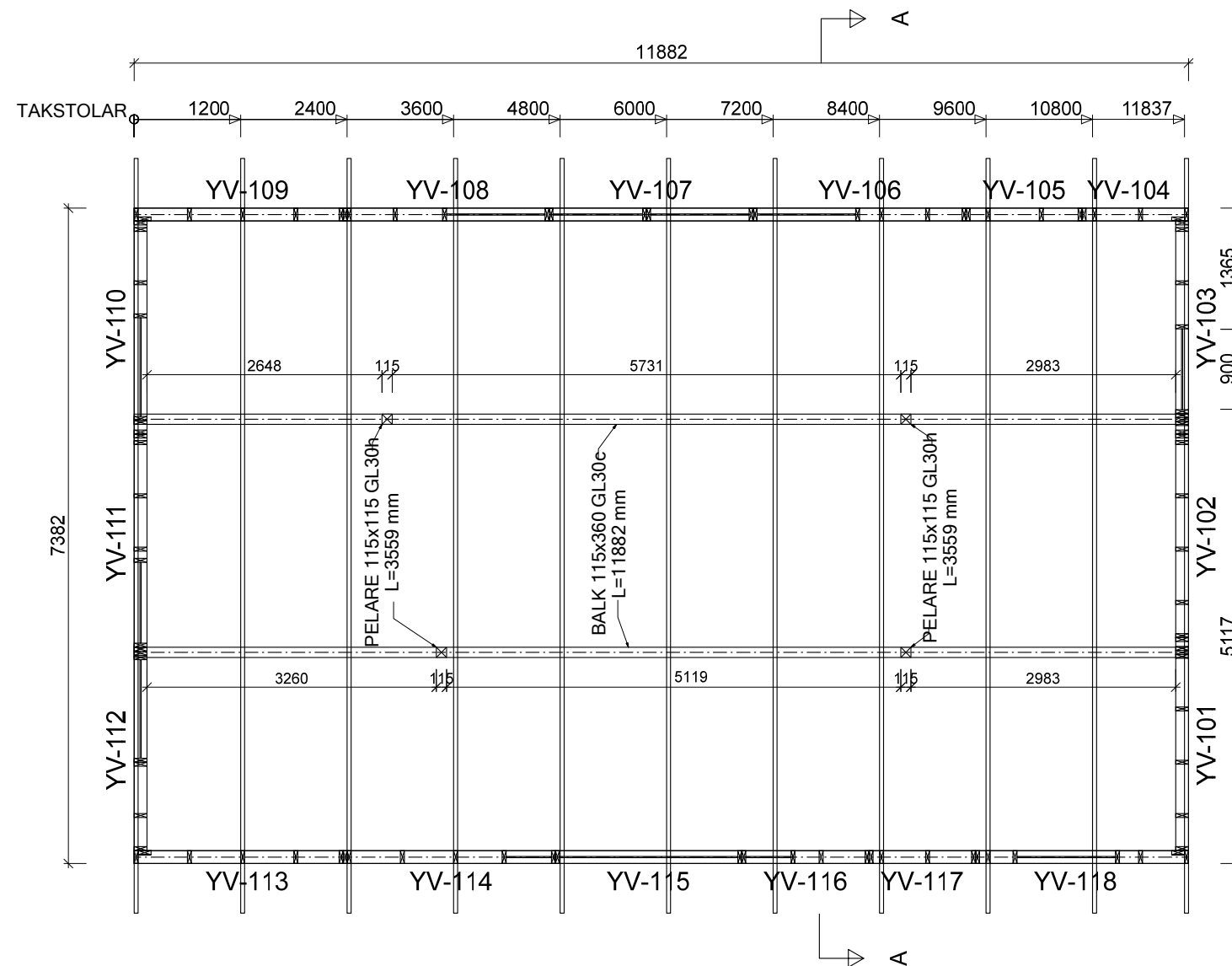
PLAN
