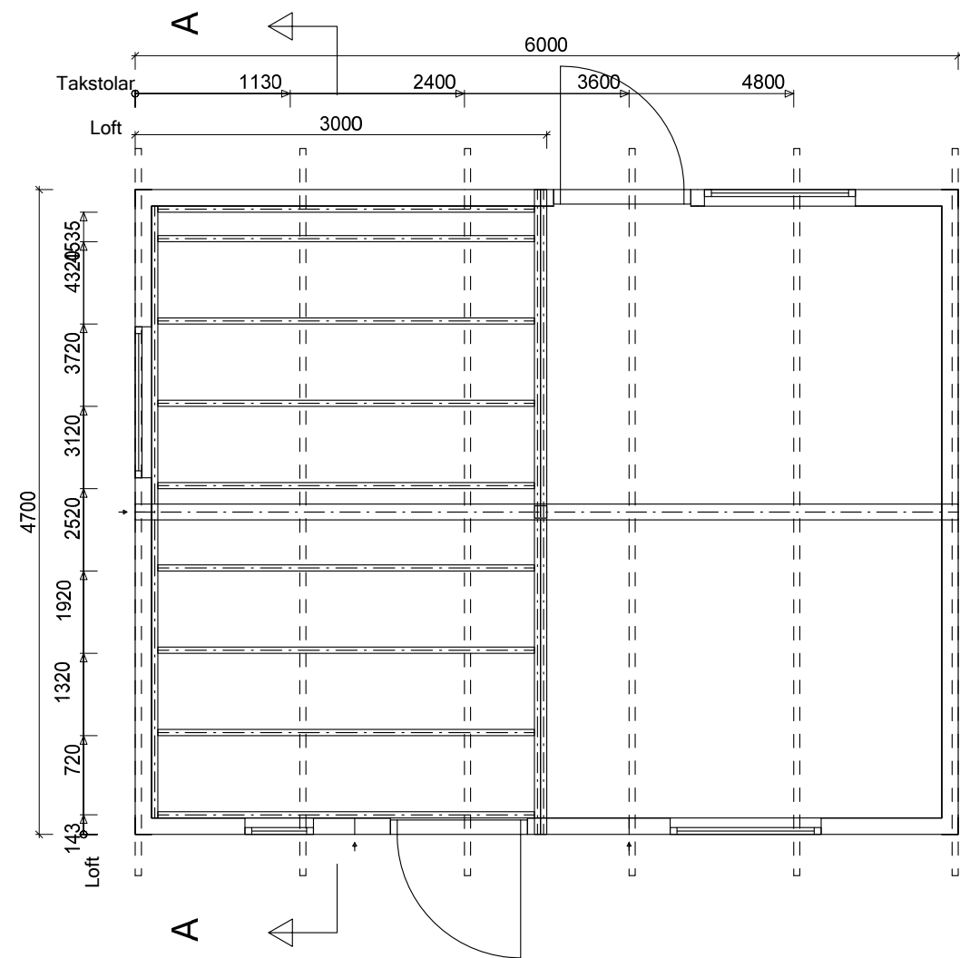
Plan
